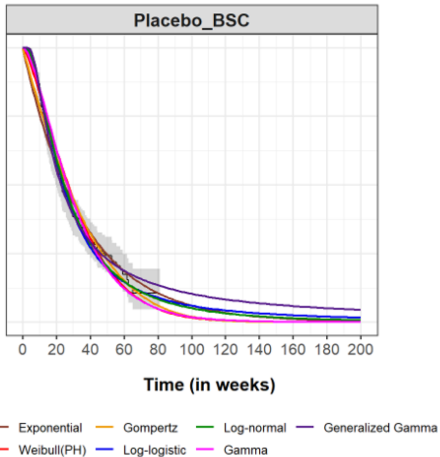
Figure 13 Extrapolated OS Individual Model and KM Data for BSC – MSM
