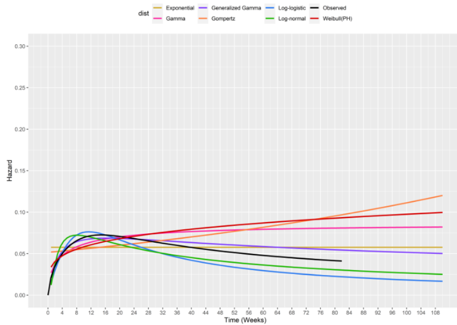
Figure 59 Smoothed hazard curves - independent fit - fruquintinib
