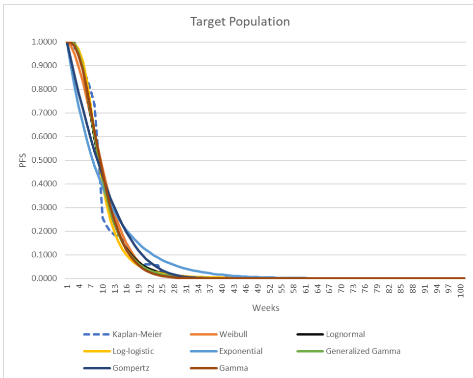
Figure 55 Extrapolated PFS individual models and KM data - BSC
