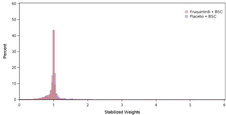
Figure 22 Histogram of stabilized weights of OS based on the MSM approach
