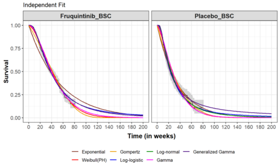
Figure 35 Extrapolated OS Individual Model and KM Data – MSM
