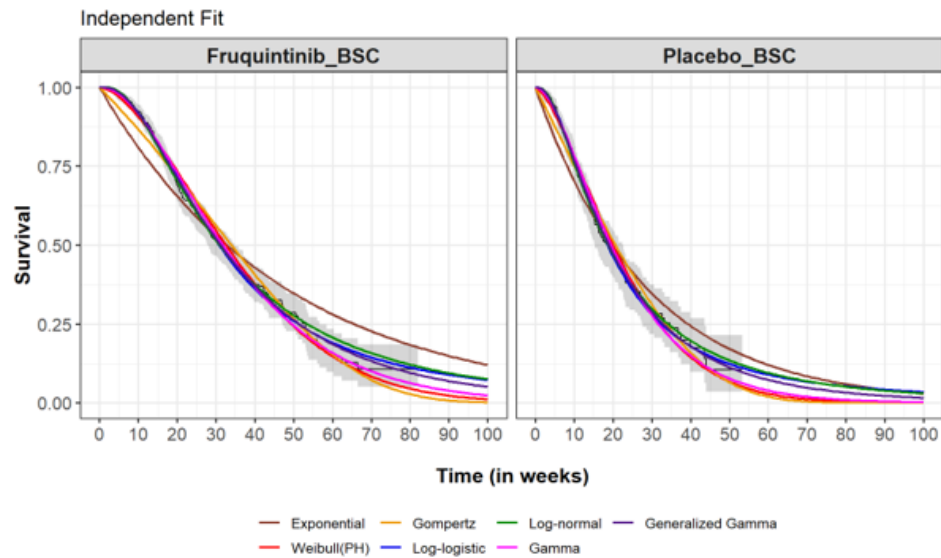
Figure 38 Extrapolated OS independent model and KM data - Naive censoring
