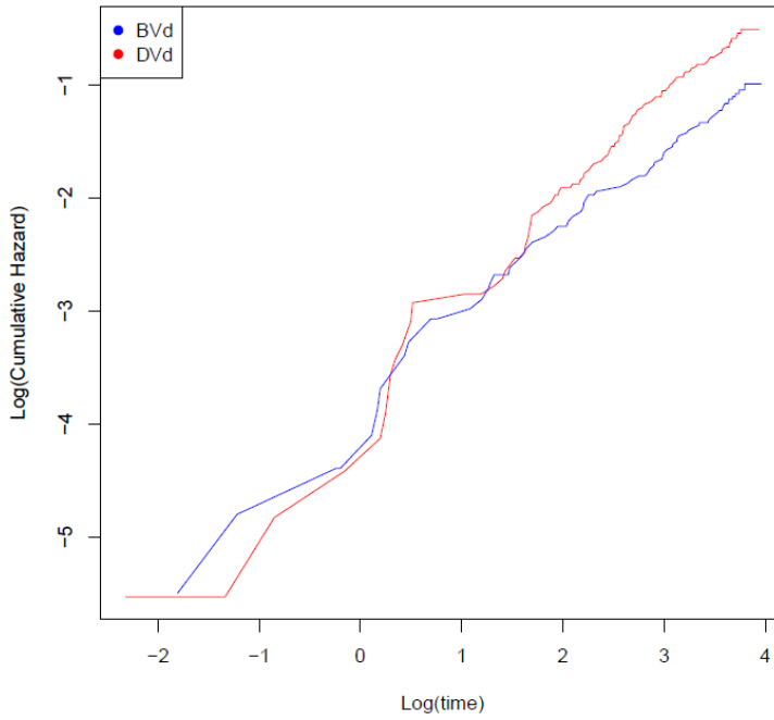
Figure 27: Plot of Log (OS Cumulative Hazard) Vs Log(Time)
