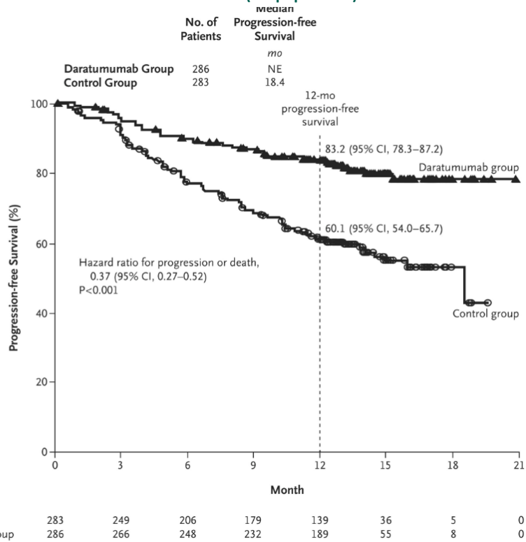
Figure 7: Kaplan-Meier Curves of PFS in POLLUX (ITT population)
