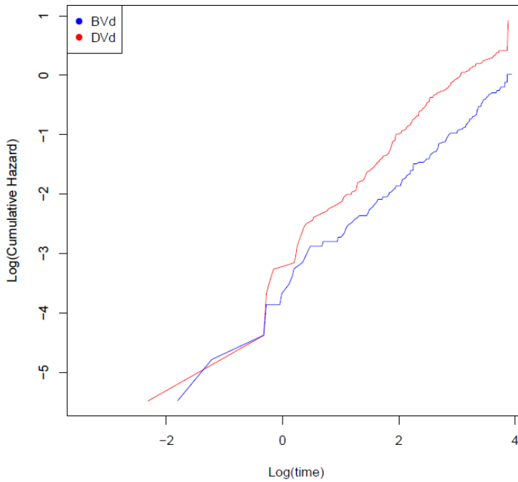
Figure 21: Plot of Log (PFS Cumulative Hazard) vs Log (Time)
