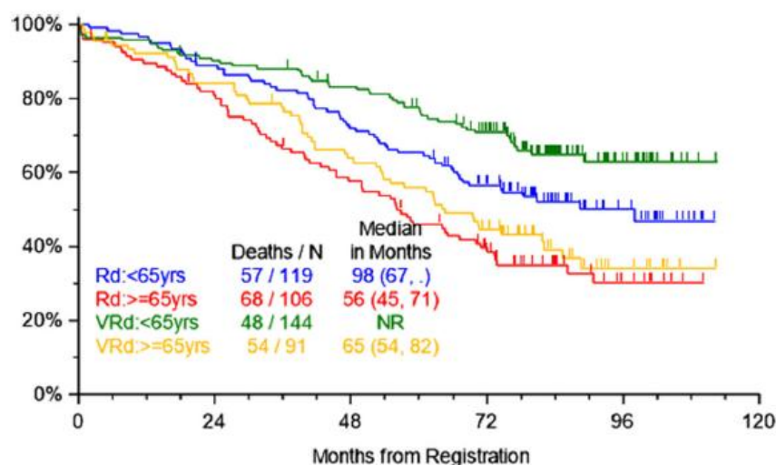
Figur 5. Kaplan-Meier OS-plot for patienter \geq 65 år, BorLenDex vs. LenDex (SWOG S0777)
