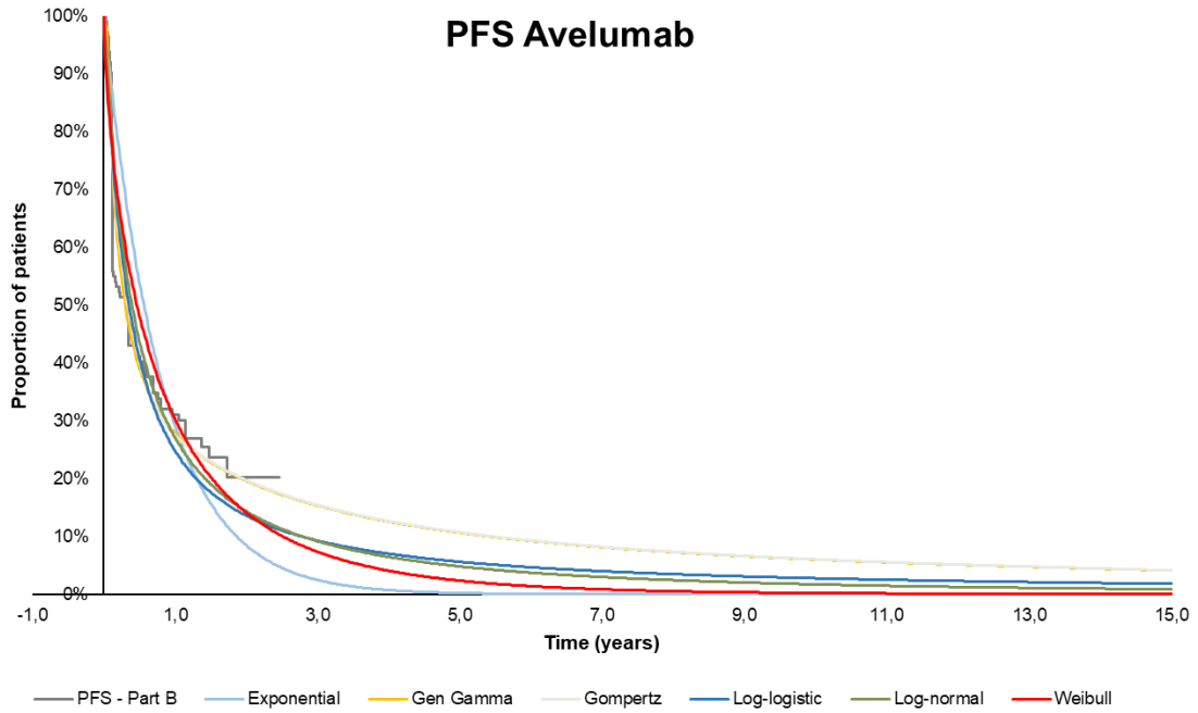
Figure 6: Curve fits - PFS Avelumab
